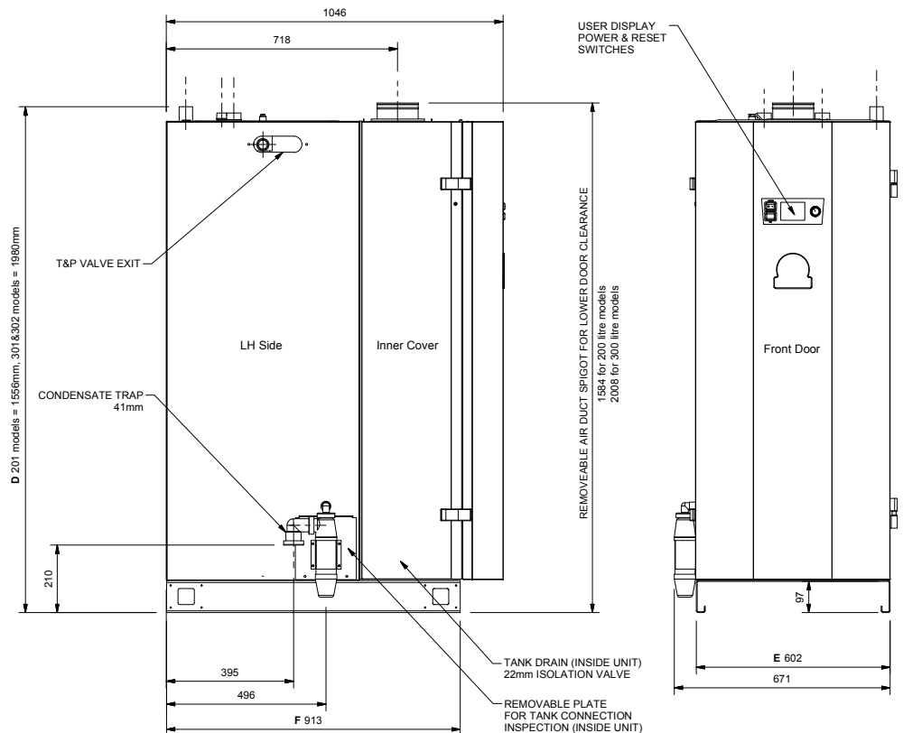
Side view
